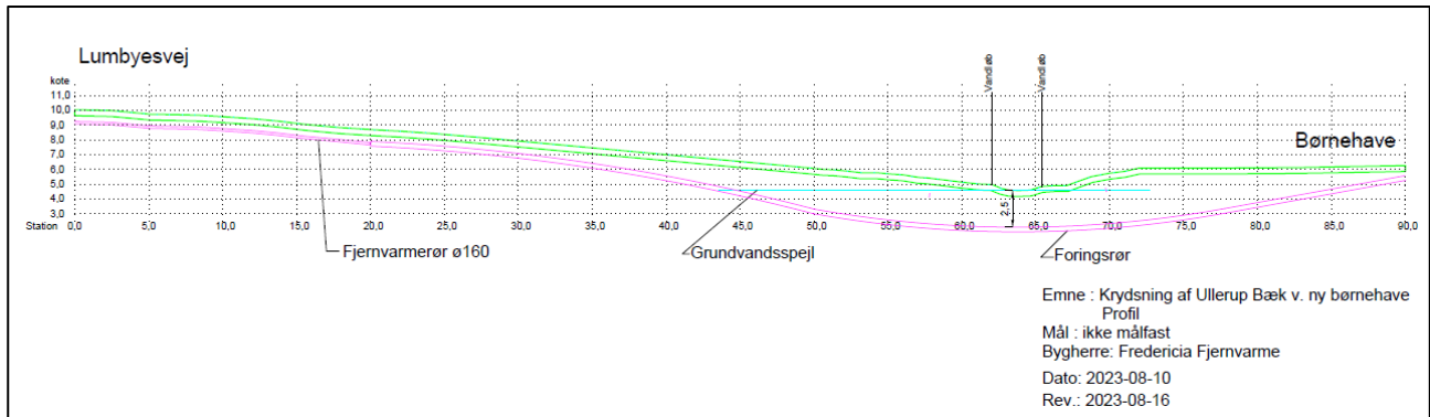
Figur 2: Profil for styret underboring.
